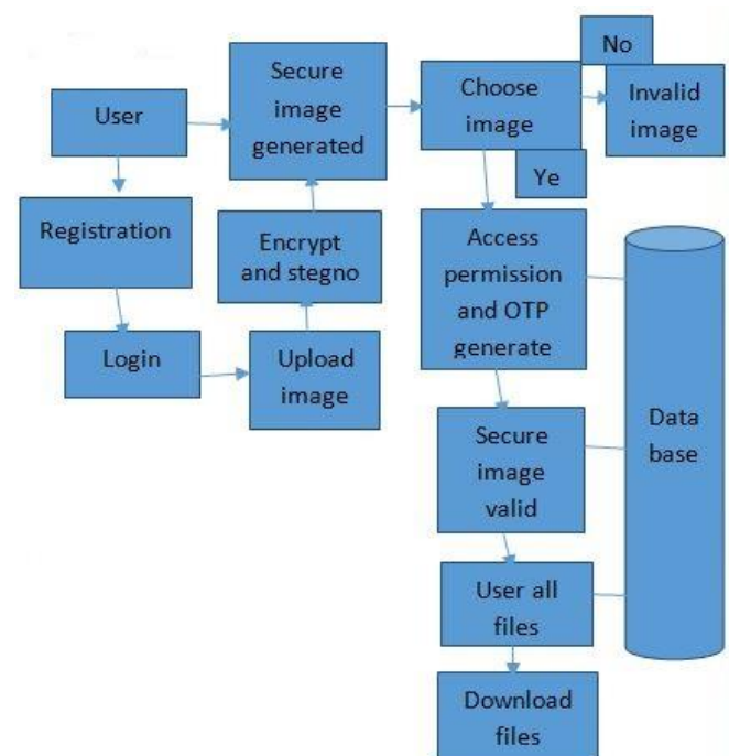
Fig1. System Architecture
